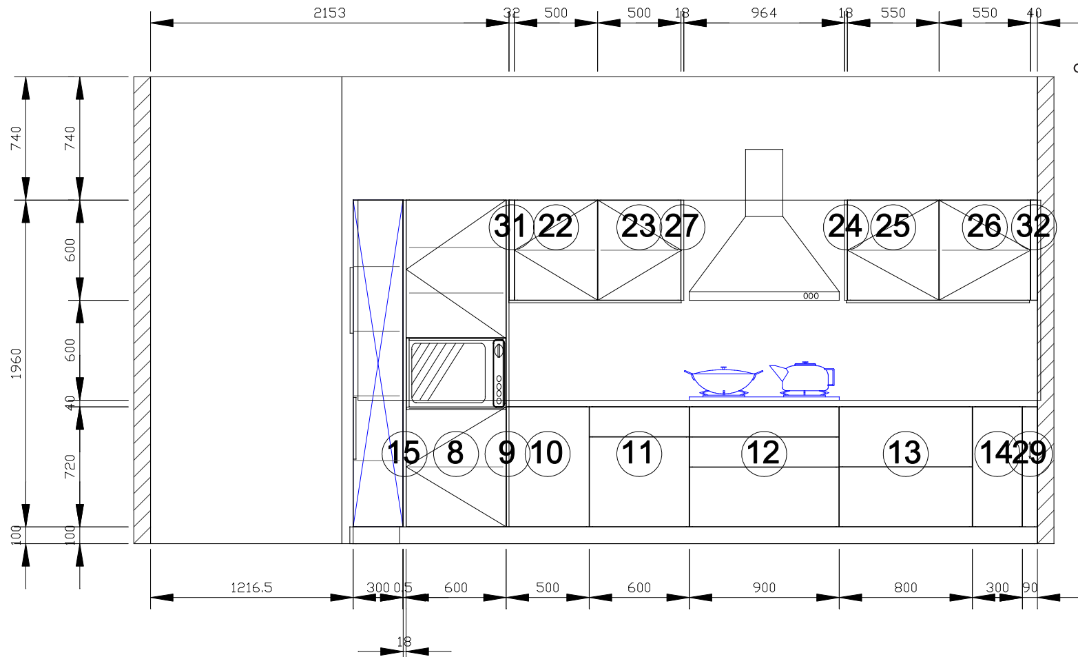
A View elevation drawing
