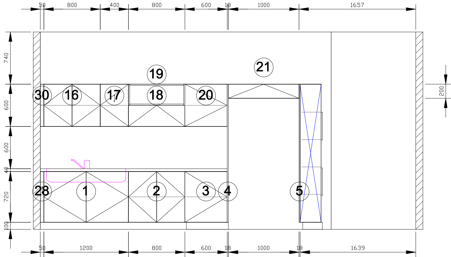
B View elevation drawing
